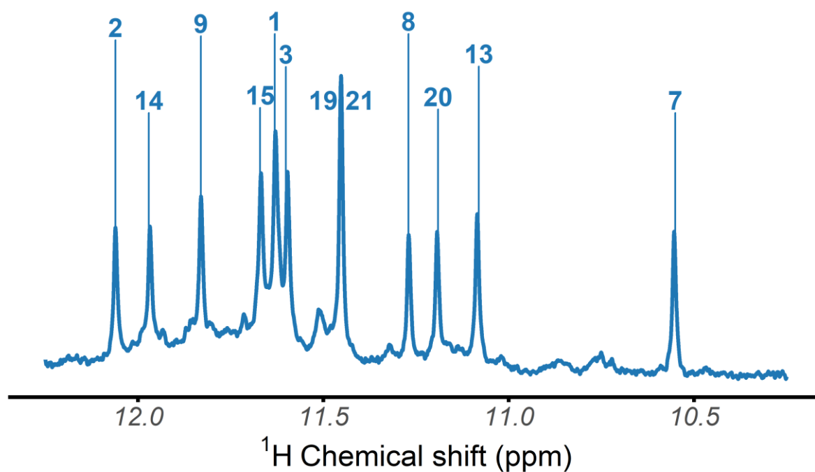
^1\text{H} -NMR spectrum of the 5Y EY oligonucleotide, acquired at 25°C in 100 mM TMAA (pH 7.0) + 1 mM KCl
