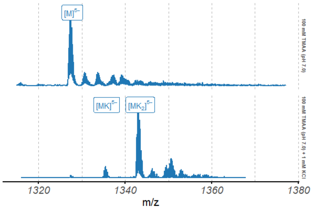
Native ESI-MS spectra of the 5Y EY oligonucleotide (10 \mu M), focused on the 5^- charge state
