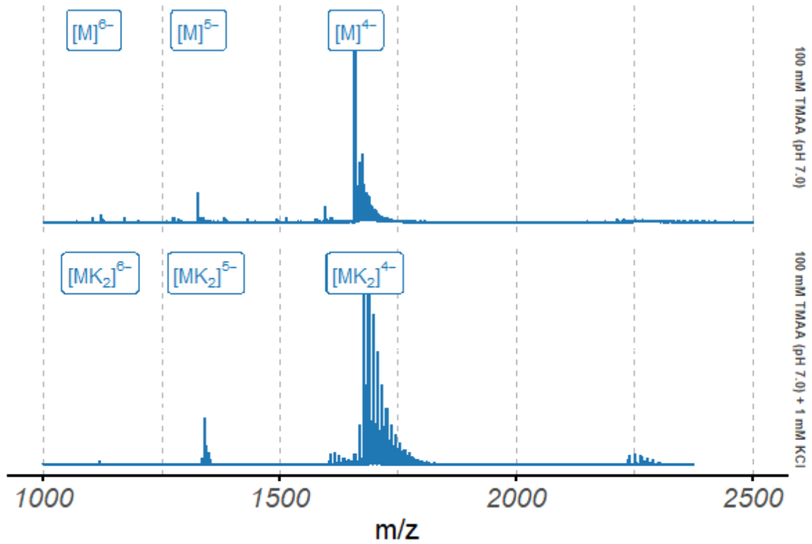
Native ESI-MS spectra of the 5Y EY oligonucleotide (10 \mu M)
