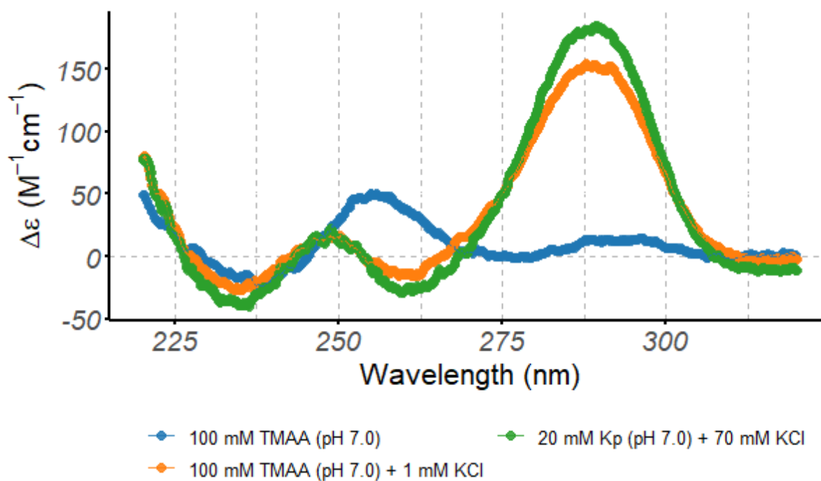
Circular dichroism spectra of the 5Y EY oligonucleotide (10 \mu M), acquired at 25°C in 0.2-cm path-length cuvettes
